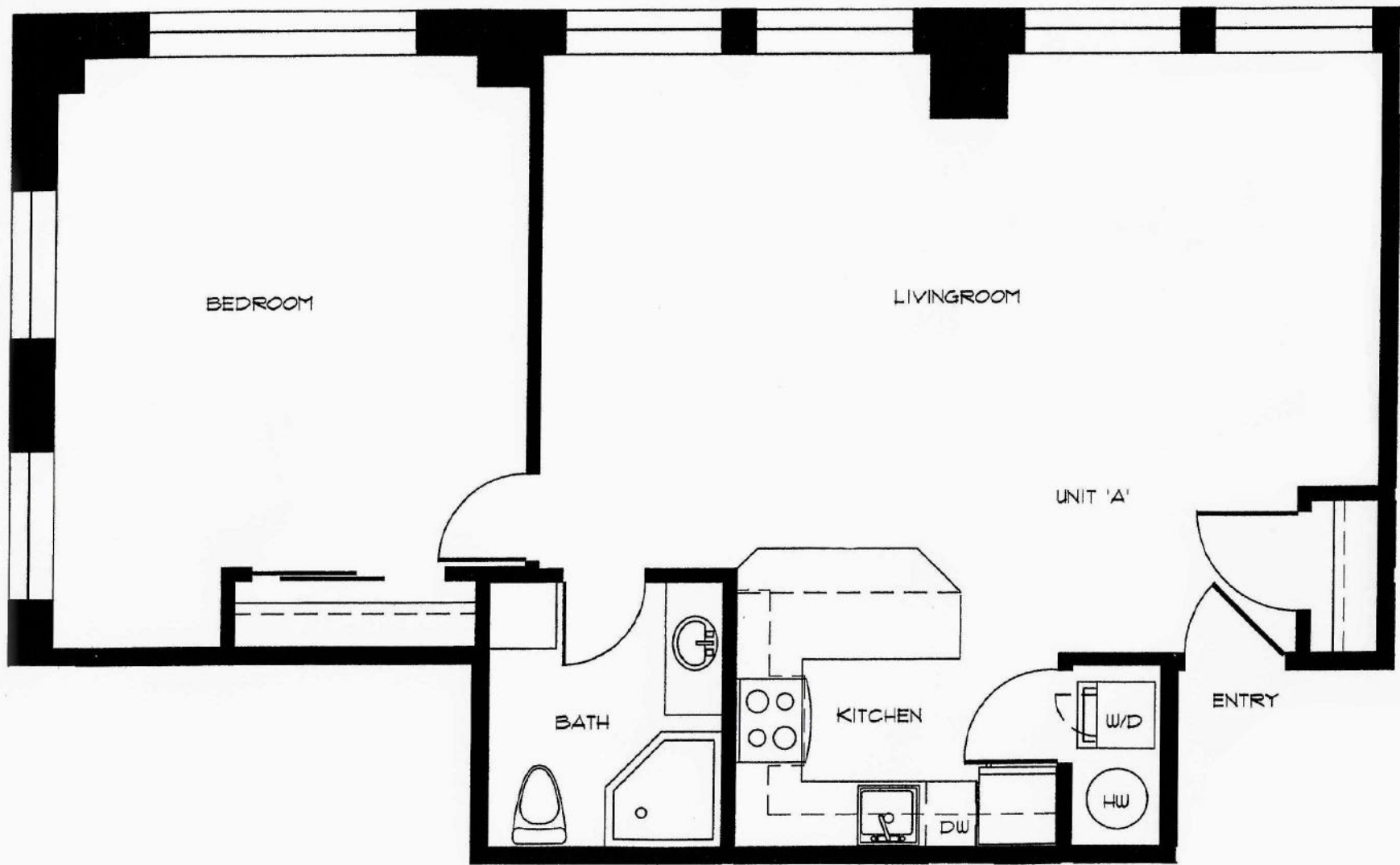
SECURITIES BUILDING LOFT UNIT 'A' - 928 S.F. 4th AND 5th FLOOR
