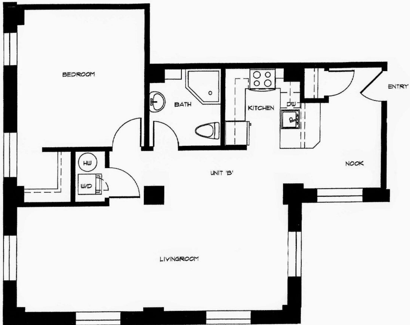
SECURITIES BUILDING LOFT UNIT 'B' - 948 SF. 4th AND 5th FLOOR
